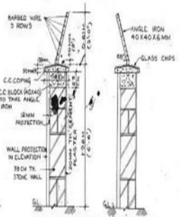
SECTION 'X-X' SECTION 'Y-Y' (FOR STONE MASONRY WALL)
