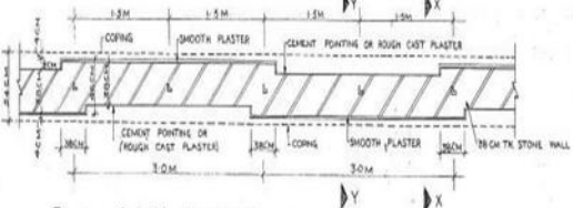
PLAN (STONE WALL)
