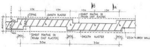
PLAN (BRICK WALL)
